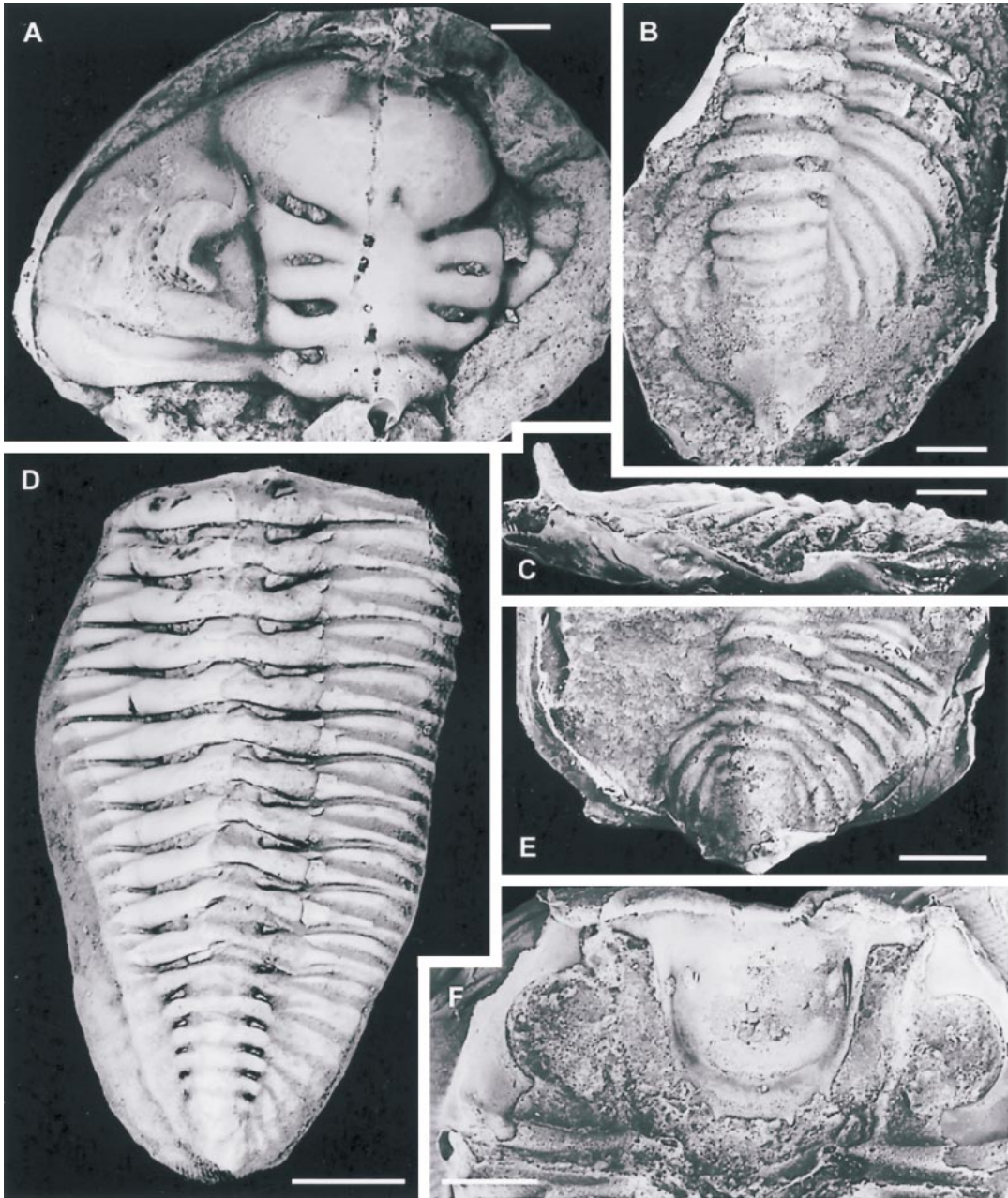
Fig. 4. Wolfartaspis liebermanii , n. sp. Icla Formation, Kochis, Cochabamba Department. All scales 5 mm. A , holotype MHNC 8132, dorsal view of cephalon, latex cast from external mold; B , C , dorsal and lateral views of pygidium, AMNH 47150, latex cast from external mold; D , dorsal view of thorax and pygidium, AMNH 47148, internal mold; E , dorsal view of pygidium and posterior part of thorax, AMNH 47151, latex cast from external mold; F , ventral view of hypostome in situ beneath cephalon, AMNH 47401, latex cast from external mold.
