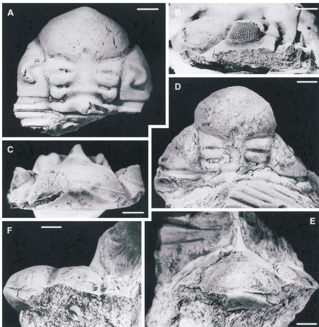
Fig. 5. Wolfartaspis lieberman , n. sp. Icla Formation, Kochis, Cochabamba Department. All scales 5 mm. A–C , dorsal, lateral, and anterior views of cephalon and part of first thoracic segment, AMNH 47403, internal mold; D–F , dorsal, anterior, and lateral views of cephalon, AMNH 47149, internal mold.
